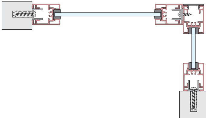
CORNER SCREEN
