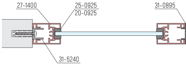
OPEN SCREEN
