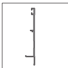
27-2180 AL27-2 CEILING MASKING STRIP, 5000 MM AN, CM
