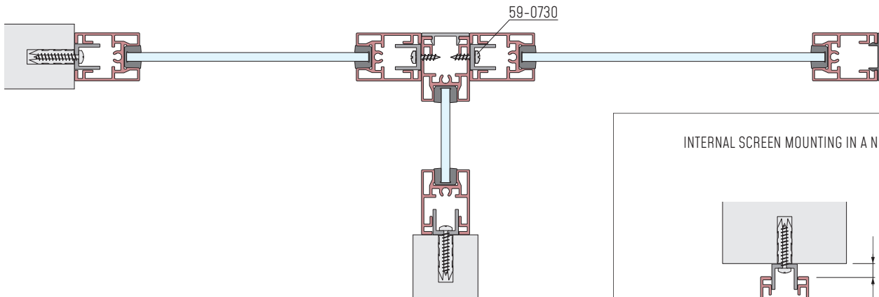
CORNER SCREEN
