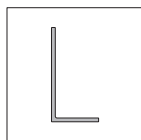
31-5250 LUMI FIXING BRACKET 50x25x2 AN, CM
