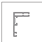
31-1603 AL31 DOOR FRAME CASING 30, 5300 MM AN, CM
