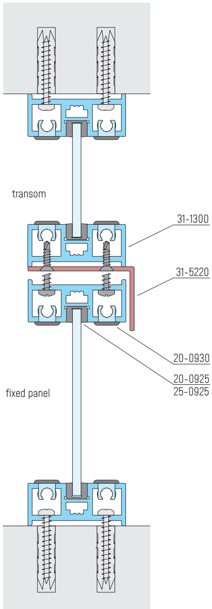
TRANSOM WITH FIXED PANEL
