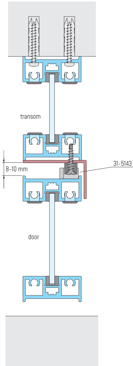
TRANSOM WITH HINGED DOORS
