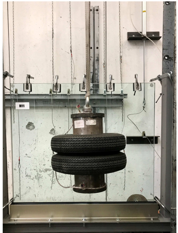
Photograph of the railing after double-tire body impact
