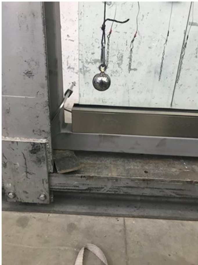
Photograph of the railing after hard body impact
