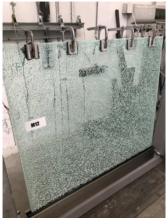
Photograph of the railing after breakage
