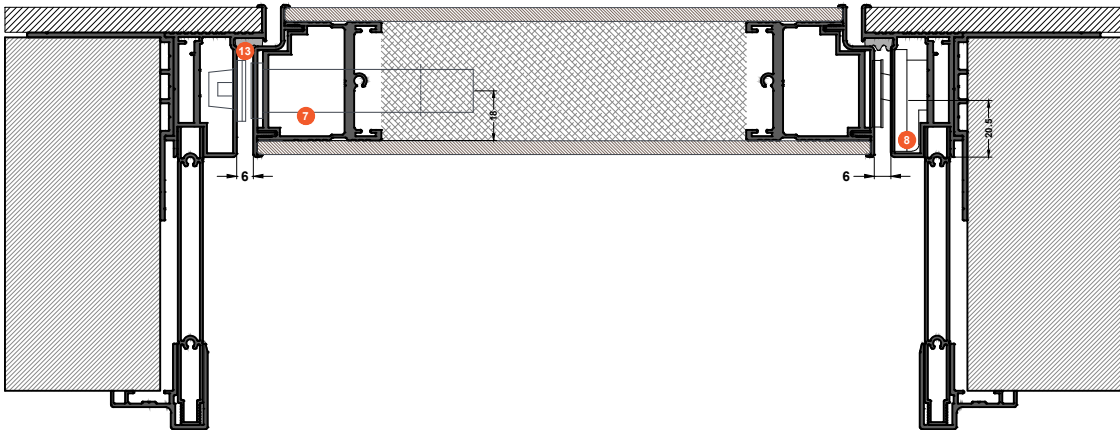
DOUBLE DOOR TOP VIEW
