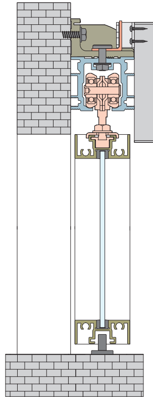
FIXED TO THE WALL
