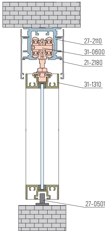
TOP TRACK WITH ROLLER AND AIR SPRING
