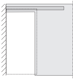
SINGLE DOOR NEXT TO THE WALL
