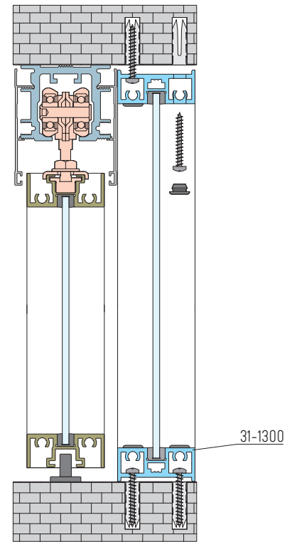
SLIDING DOOR AND FIXED PANEL
