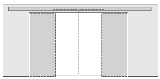
DOUBLE DOOR WITH TWO FIXED PANELS
