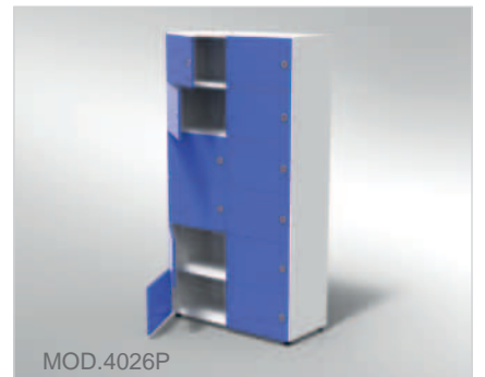
■ CABINET 12 DOORS 12 COMPARTMENTS ■ DIMENSIONS: 104x46x200h.
